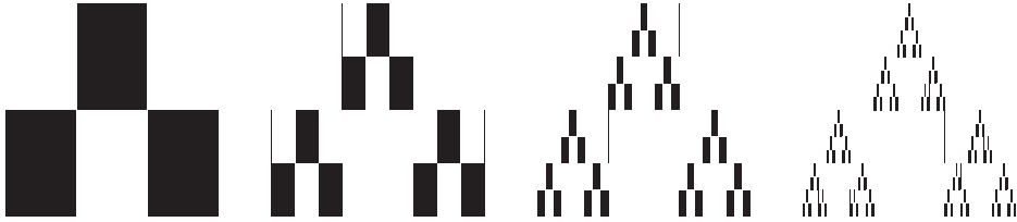
FIGURE 1. First four generations of a Bedford–McMullen carpet.
