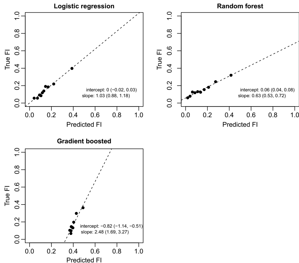
Figure 2. Calibration statistics for logistic regression, random forest, and gradient boosted model in test set to predict food insecurity. Legend: FI = food insecurity.
