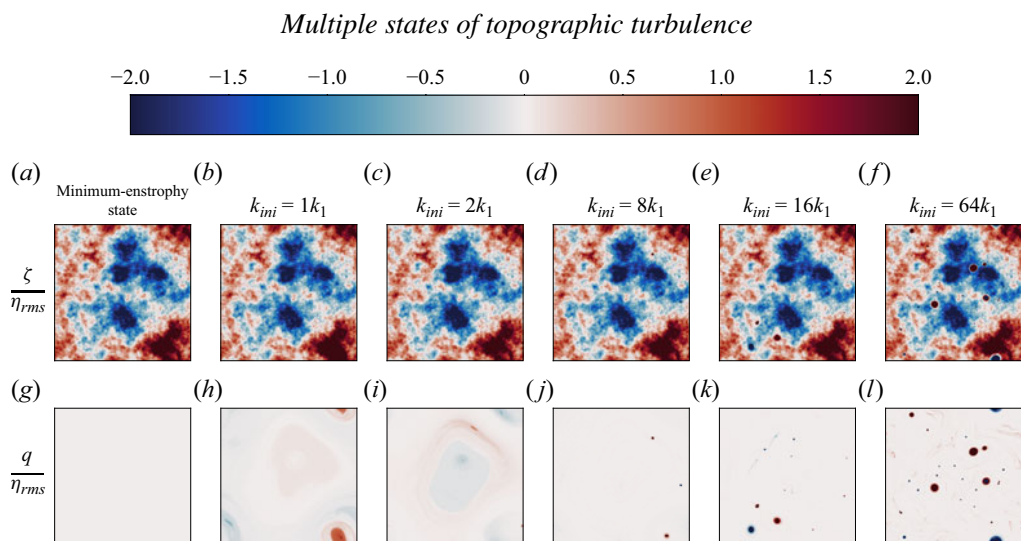
Figure 6. Long-term snapshots of E_{\#} runs for k_{ini} = [1, 2, 8, 16, 64]k_1 (second–sixth columns) compared with the minimum-ensrophy state at the same energy level (first column): first row, \zeta/\eta_{rms} ; second row, q/\eta_{rms} .
