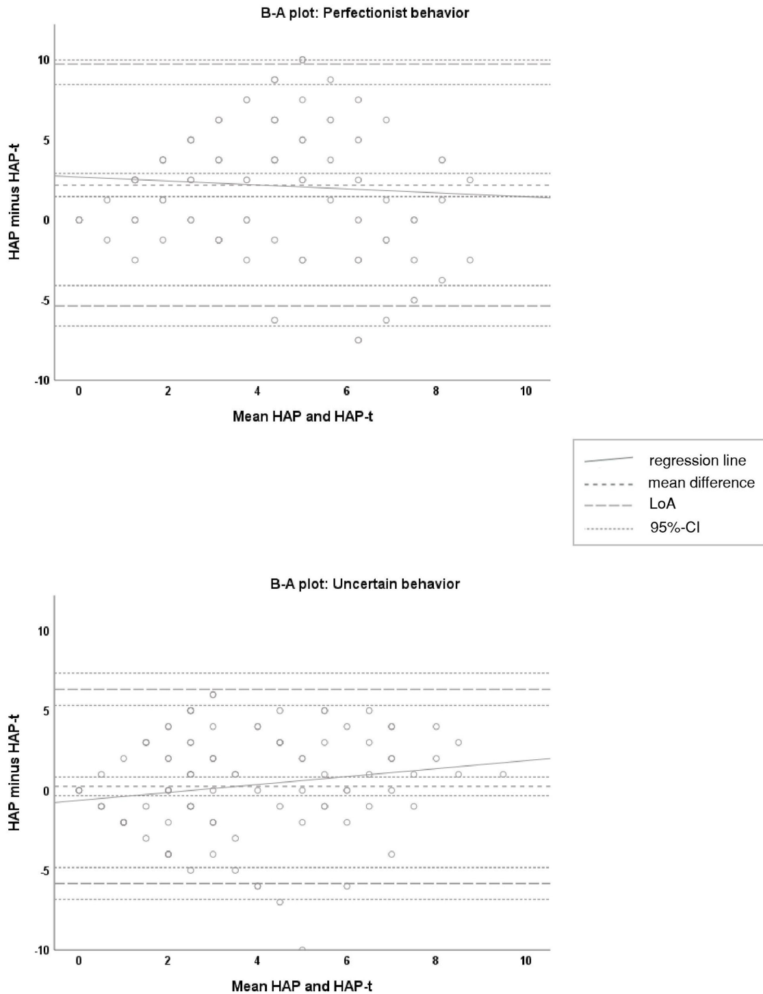
Figure 2. Bland and Altman plots: HAP-HAP-t differences for PERF and UNC. Note: relative scores (0–10); x = (HAP + HAP-t)/2 , y = HAP - HAP-t ; LoA (limits of agreement) = mean difference \pm (1.96*standard deviation); 95% CI (95% confidence intervals) = \pm (standard error*t value for degrees of freedom).
