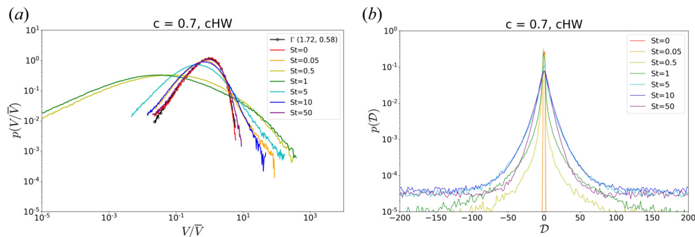
FIGURE 15. (a) PDF of volume normalised by the mean ( V/\bar{V} ) and (b) PDF of impurity velocity divergence D for different Stokes numbers for ^{184}\text{W}^{1+} ( \alpha = 0.01 ) in the quasi-adiabatic regime ( c = 0.7 , cHW model).
