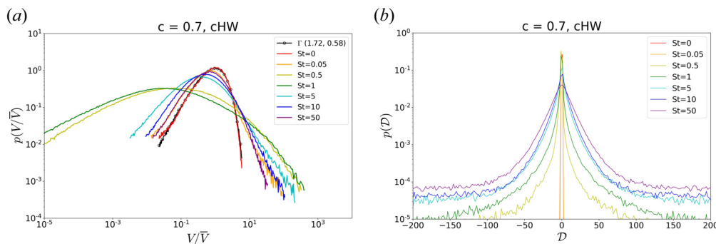
FIGURE 16. (a) PDF of volume normalised by the mean ( V/\bar{V} ) and (b) PDF of the impurity velocity divergence D for different Stokes numbers for ^{184}\text{W}^{44+} ( \alpha = 0.48 ) in the quasi-adiabatic regime ( c = 0.7 , cHW model).
