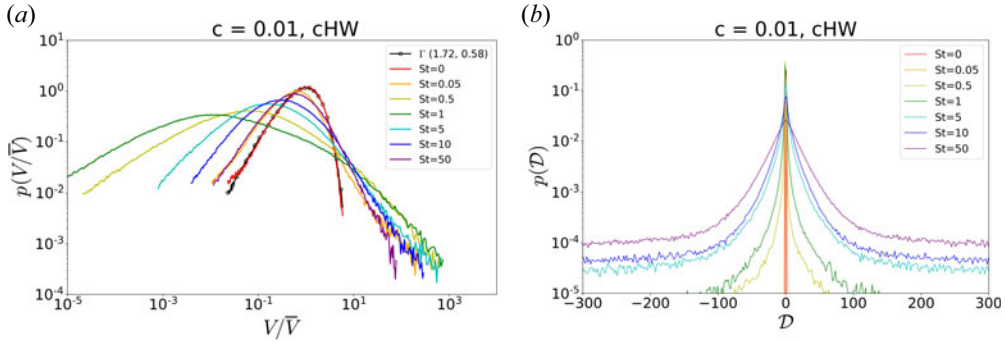
FIGURE 10. (a) PDF of volume normalised by the mean ( V/\bar{V} ) and (b) PDF of impurity velocity divergence D for different Stokes numbers for ^{184}\text{W}^{20+} ( \alpha = 0.22 ) in hydrodynamic regime ( c = 0.01 , cHW model).
