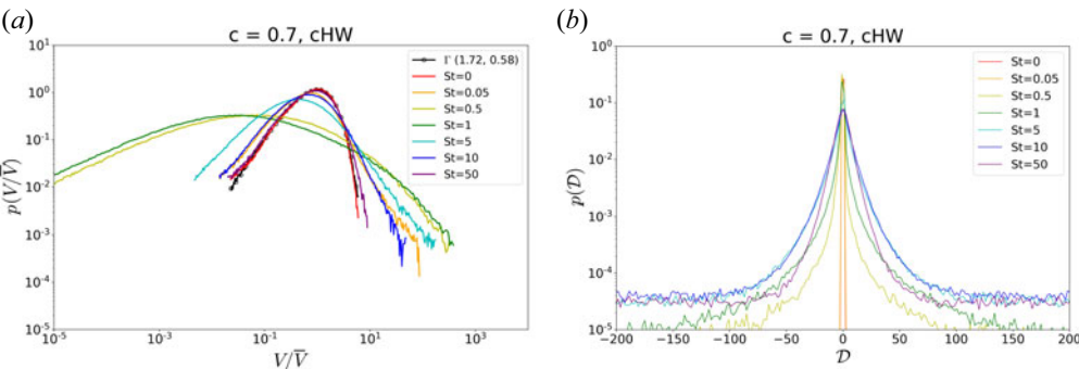
FIGURE 15. (a) PDF of volume normalised by the mean ( V/\bar{V} ) and (b) PDF of impurity velocity divergence \mathcal{D} for different Stokes numbers for ^{184}\text{W}^{1+} ( \alpha = 0.01 ) in the quasi-adiabatic regime ( c = 0.7 , cHW model).
