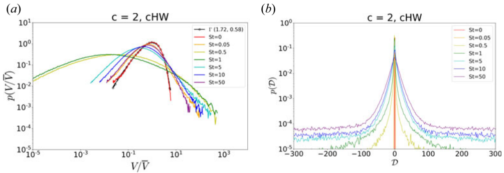
FIGURE 11. (a) PDF of volume normalised by the mean ( V/\bar{V} ) and (b) PDF of impurity velocity divergence D for different Stokes numbers for ^{184}\text{W}^{20+} ( \alpha = 0.22 ) in hydrodynamic regime ( c = 2 , cHW model).
