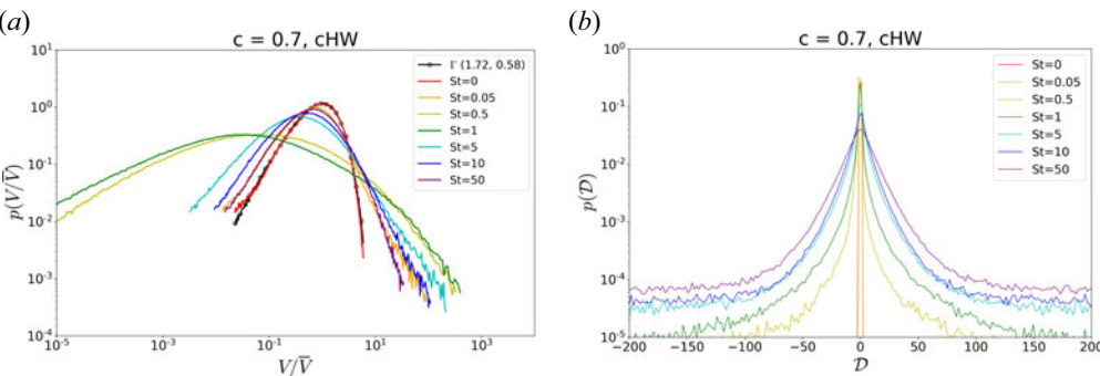
FIGURE 16. (a) PDF of volume normalised by the mean ( V/\bar{V} ) and (b) PDF of the impurity velocity divergence \mathcal{D} for different Stokes numbers for ^{184}\text{W}^{44+} ( \alpha = 0.48 ) in the quasi-adiabatic regime ( c = 0.7 , cHW model).
