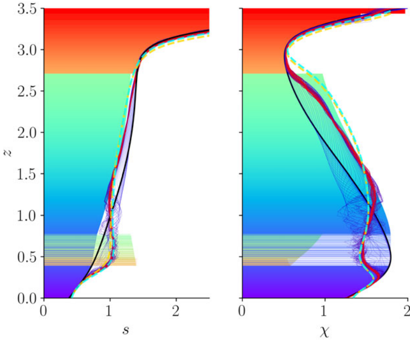
FIGURE 29. Horizontally averaged profiles of s and \chi plotted at intervals of 1 code time unit, between t = 0 (blue) to t = 600 (red), for the simulation visualised in figure 28 . Also plotted are the profiles obtained by taking expectation values of \mathcal{P}(m, \mu) (gold dashed line) and from (5.13) and (5.14) (cyan dashed line).
