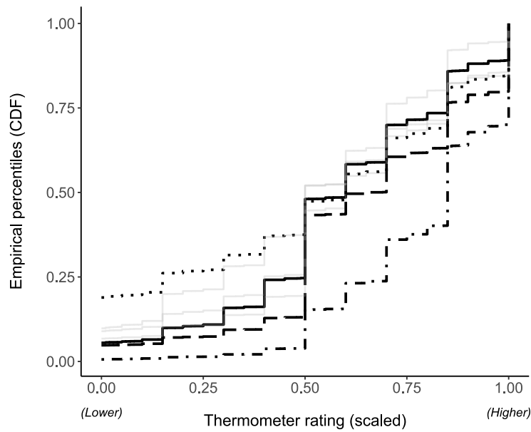
Figure 1: ANES 2020: Empirical cumulative distribution function (ECDF). Highlighted variables: Feminists (solid line, —), Gay men and Lesbians (dashed line, ---), BLM movement (dotted line, .....), and Scientists (dash-dot line, -.-.).
