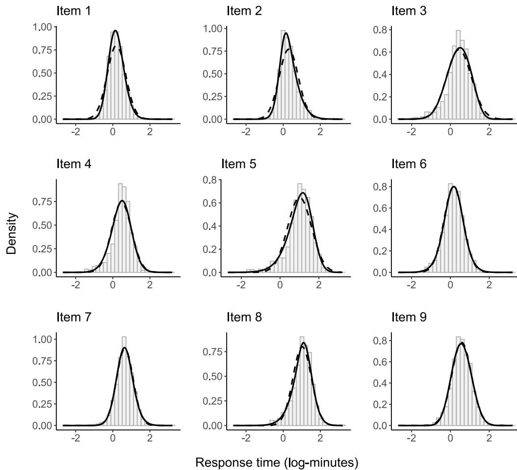
Figure 3: PISA 2018: Empirical and model-implied marginal distributions for response times (in log-minutes). The solid line (—) is the SN model, and the dashed line (---) the Normal model.
