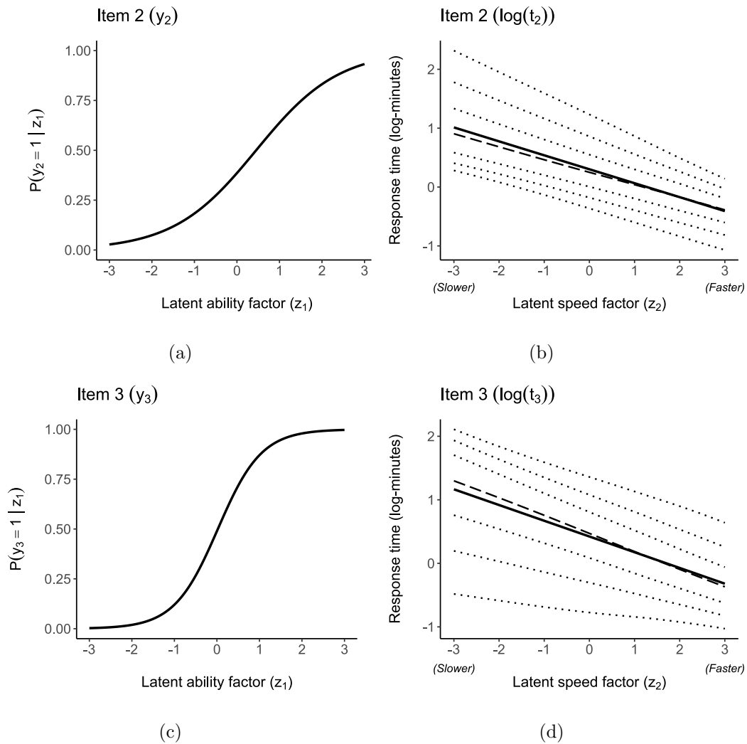
Figure 4: PISA 2018: Fitted conditional expected values (solid line, —), median (dashed line, ---), and percentiles (dotted lines, ..... ) for IR and log-RT for items 2 and 3.
