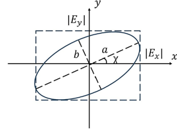
Figure 2. Polarization ellipse.
