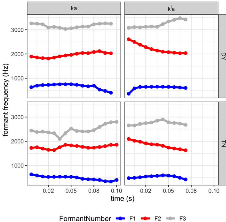
Figure 2. (Colour online) The first, second and third formant frequency trajectories for syllables /kà/ and /k'jà/. The syllable /kà/ is taken from the disyllabic word 'favorite' (TN: [kà ɕóʔ] and DY: [kà ɕò:]). The syllable /k'jà/ is taken from the disyllabic word 'China' ([k'jà náʔ]). One example token for each speaker and each consonant category is selected for the illustration.
